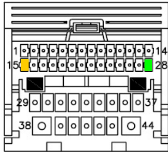
Radio connector Rear view
